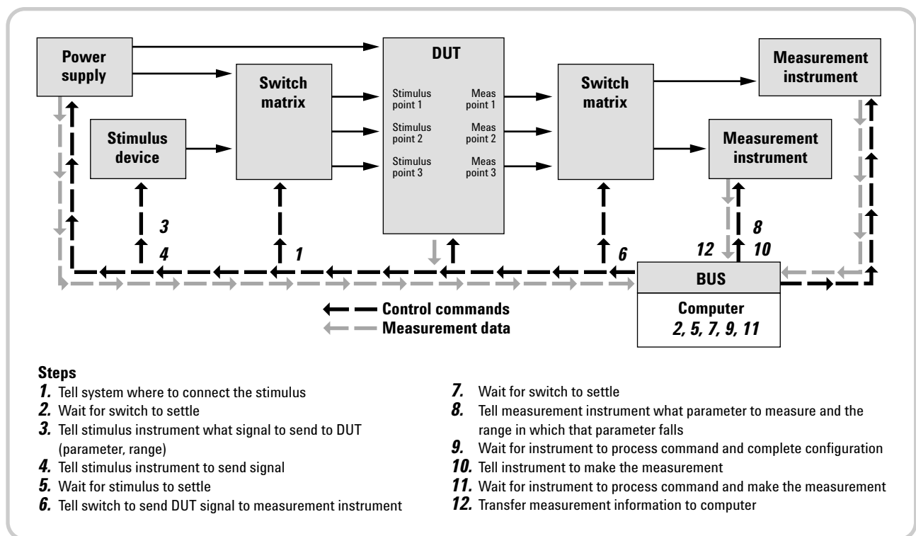
Figure 1. Steps involved in making measurements with a typical computer-controlled system.
