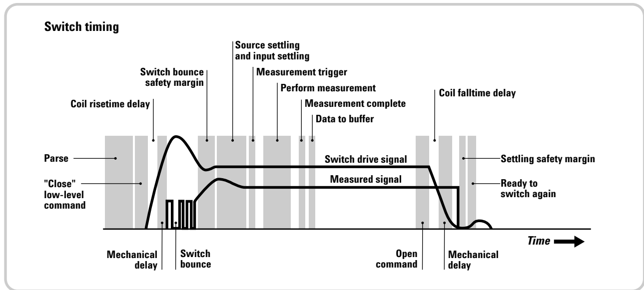
Figure 6. This diagram shows what happens when you tell a switch to close, take a measurement, and then reopen. The "switch drive signal" represents the actual voltage that causes the switch to change states. The resulting "measured signal" is connected from the DUT to the measurement instrument.
