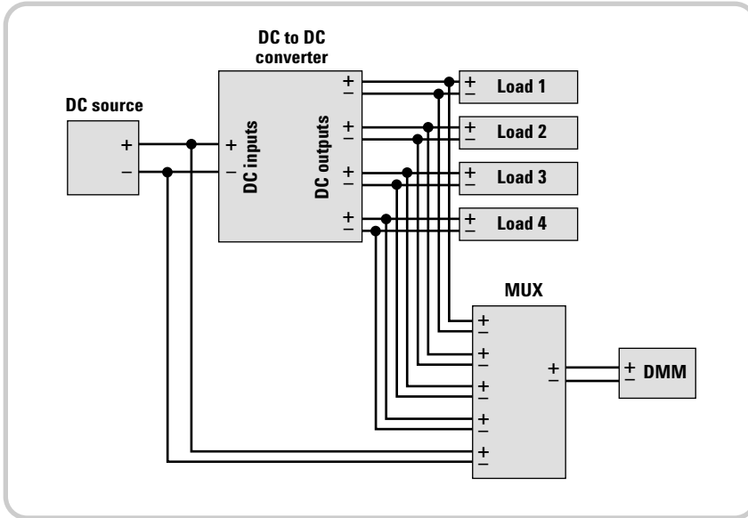
Figure 4. Testing a four-output DC-to-DC converter with a single DMM requires a complex multiplexing scheme and can involve significant delays.
