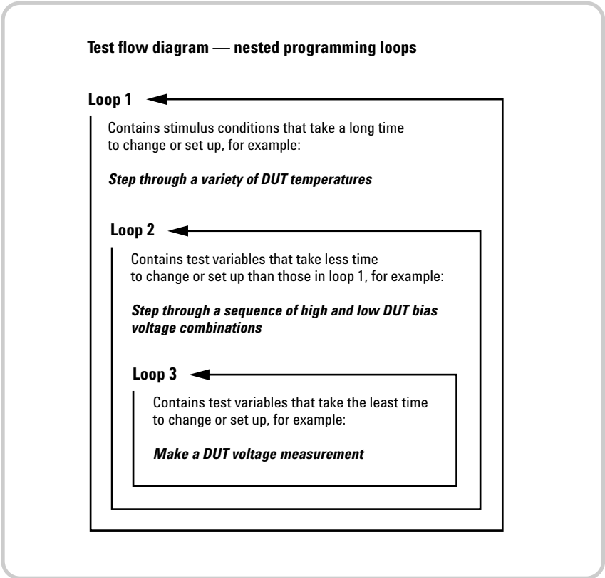
Figure 7. To minimize overall test time, structure test loops so that the most time-consuming operations are performed the fewest number of times.
