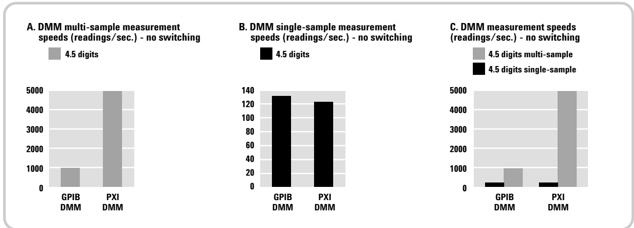
Figure 3. Burst speed can be misleading. This diagram compares multi-sample and single-sample 4.5-digit measurements made with a GPIB DMM and PXI DMM. "C" combines "A" and "B" on the same scale.
