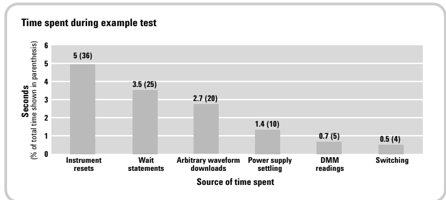
Figure 2. Hierarchy of delays in a typical test plan
